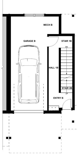
2 GROUND LEVEL - MRKG - LOT 11 A2.5 / 1/4" = 1'-0"
